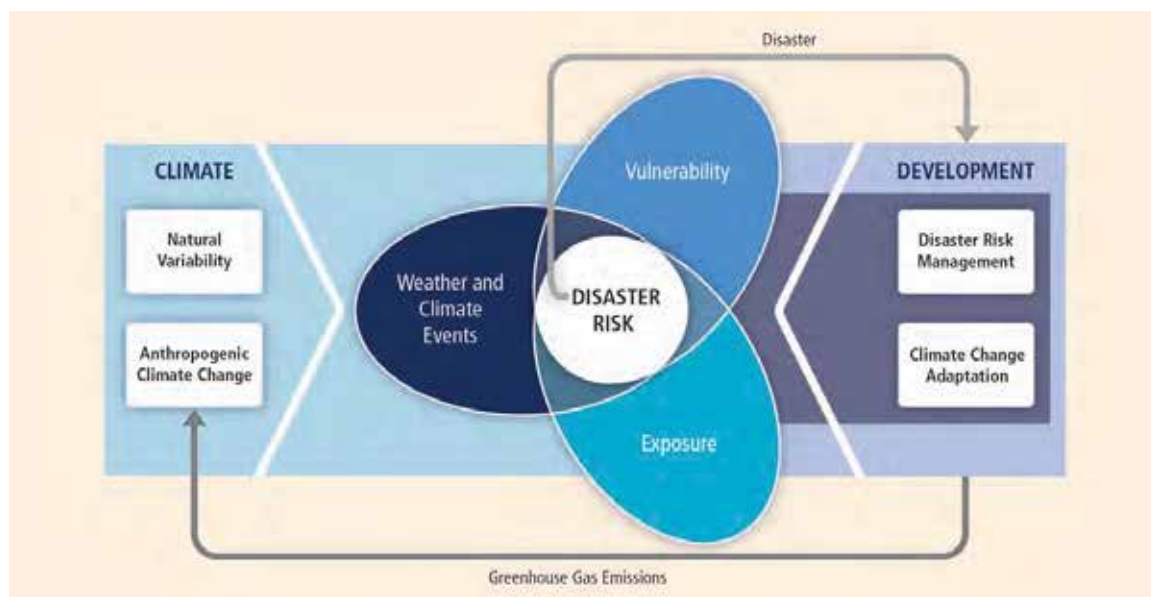
Figure 1: Core concepts of Special Report on Managing the Risks of Extreme Events and Disasters to Advance Climate Change Adaptation (SREX)
