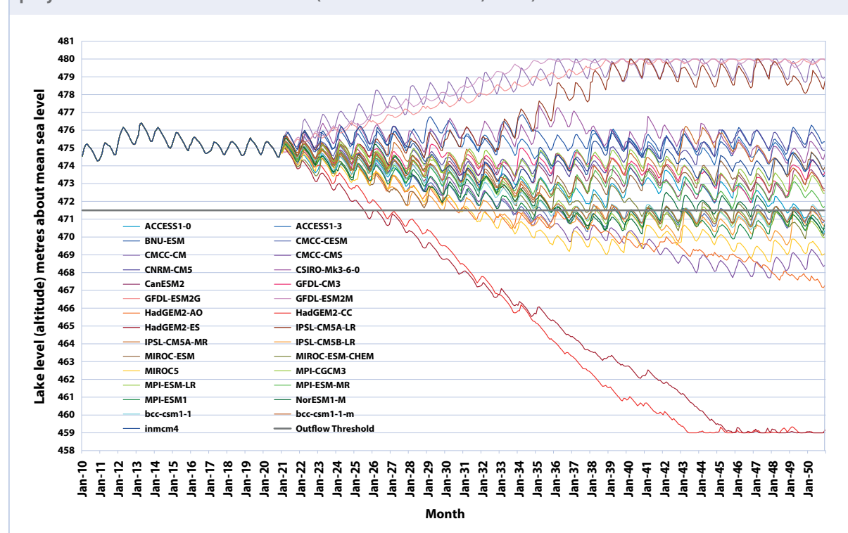
Figure 3: Climate change impacts on Lake Malawi levels based on 29 Global Climate Model projections in the Shire River Basin. (Source: Bhawe et al., 2019)
