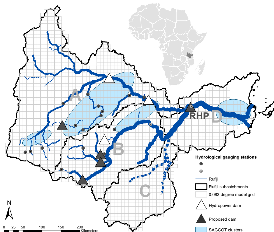
Figure 4: Hydrological model of the Rufiji system overlaid with 0.083 ° (~9 by 9km) grid and areas identified for irrigation expansion (SAGCOT clusters) (Siderius et al., 2018). RHP is Rufiji Hydropower Project. Letters refer to main tributaries: A is Great Ruaha, B is Kilombero, C is Luwegu and D is the Main Rufiji channel. (Source: Conway et al., 2019)
