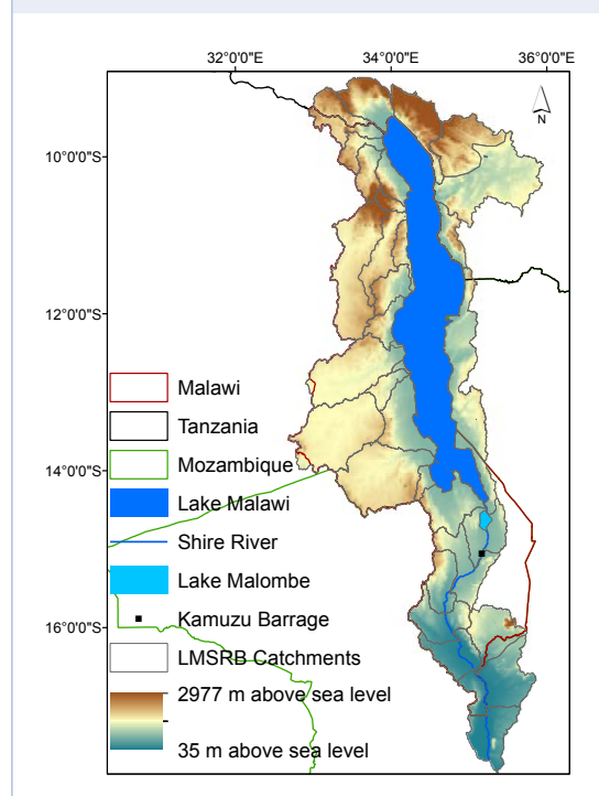
Figure 2: Location, elevation and catchments of the Lake Malawi Shire River Basin. (Source: Bhawe et al., 2019)
